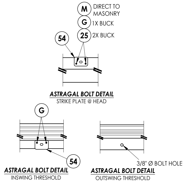
HARDWARE DETAILS
