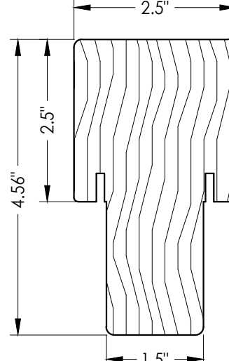
4 WOOD MULLION ENDURA FrameSaver
