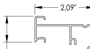
16 INSWING SIDELITE BASE ENDURA
