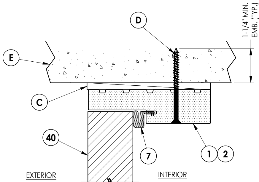
2 10 VERTICAL CROSS SECTION Outswing Shown (Inswing Similar) Shown Direct to Masonry
