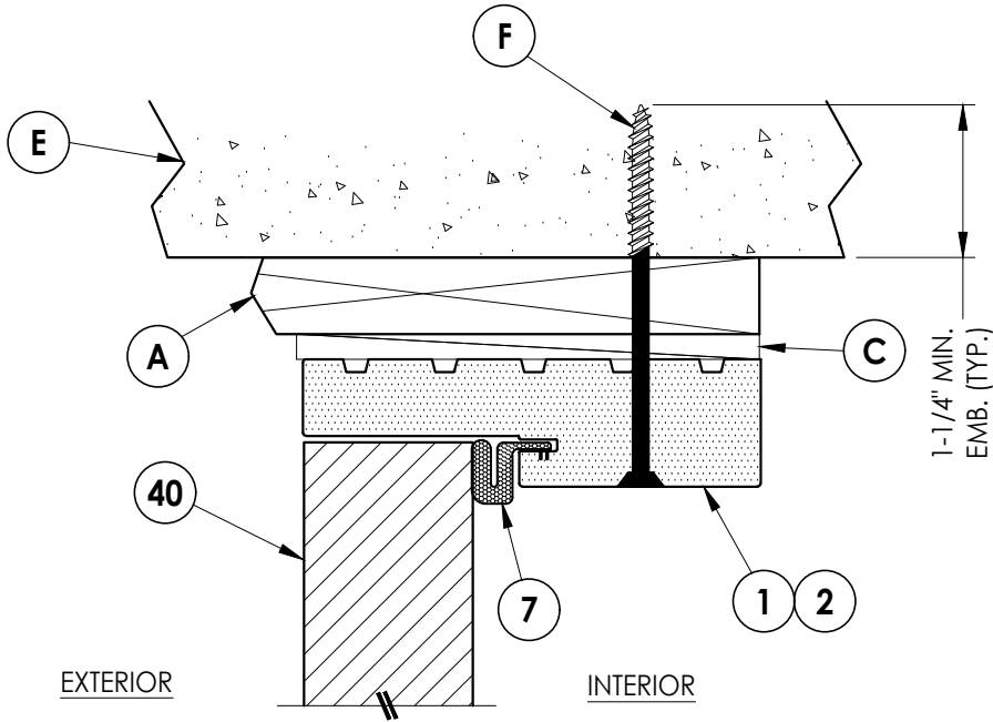
2 VERTICAL CROSS SECTION 9 Outswing Shown (Inswing Similar) Shown w/ 1X Buck
