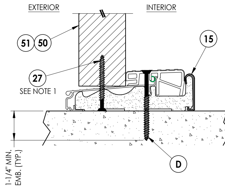
4 11 VERTICAL CROSS SECTION Outswing Sill
