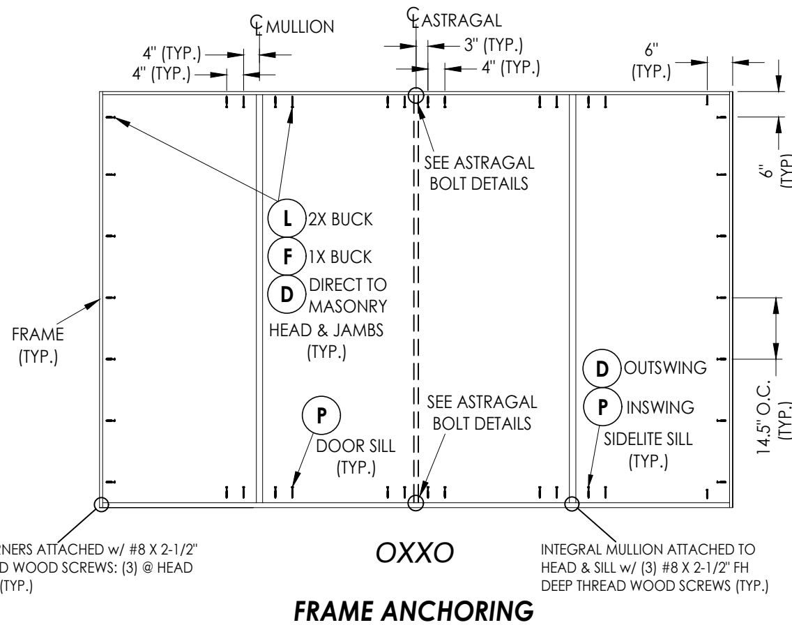
OXXO 2X BUCK ANCHORING
