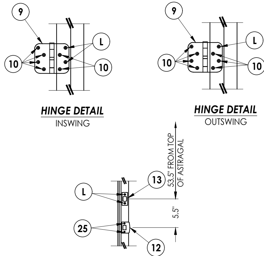
LATCH & DEADBOLT STRIKE PLATE DETAILS
